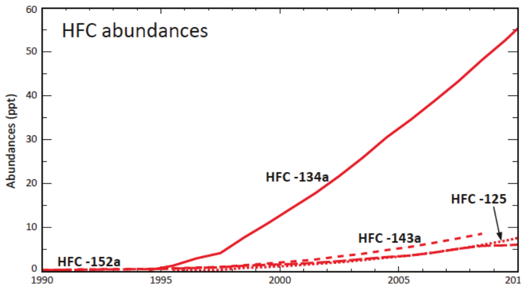
Figure 2: Global average atmospheric abundances of four major HFCs used as ODS replacements since 1990
