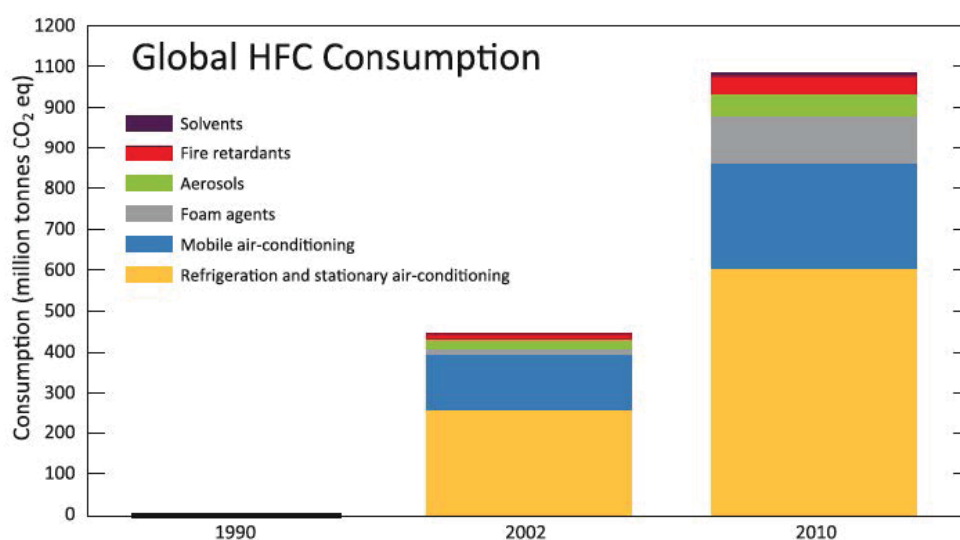
Figure 3: Global HFC consumption.
