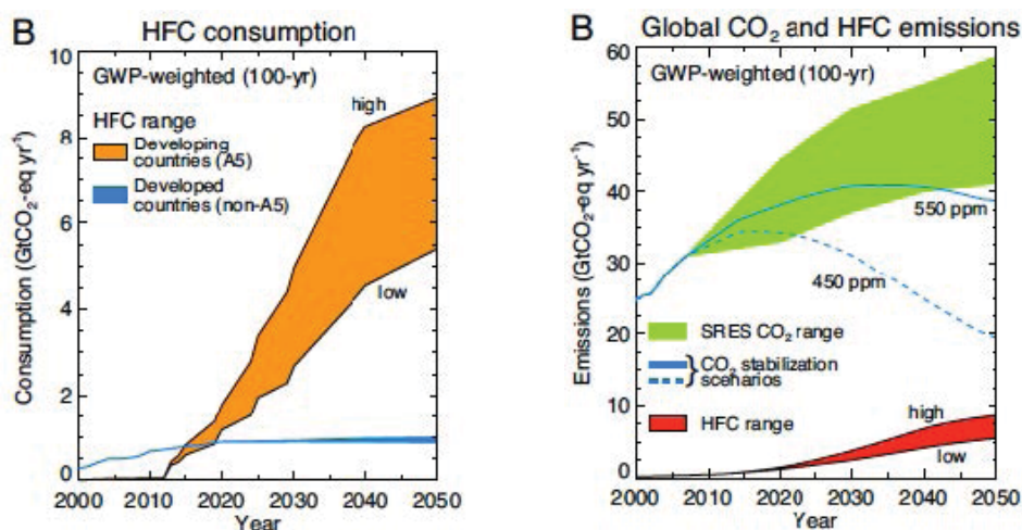
Figure 4: Projected HFCs consumption and emissions by Velders et al.
