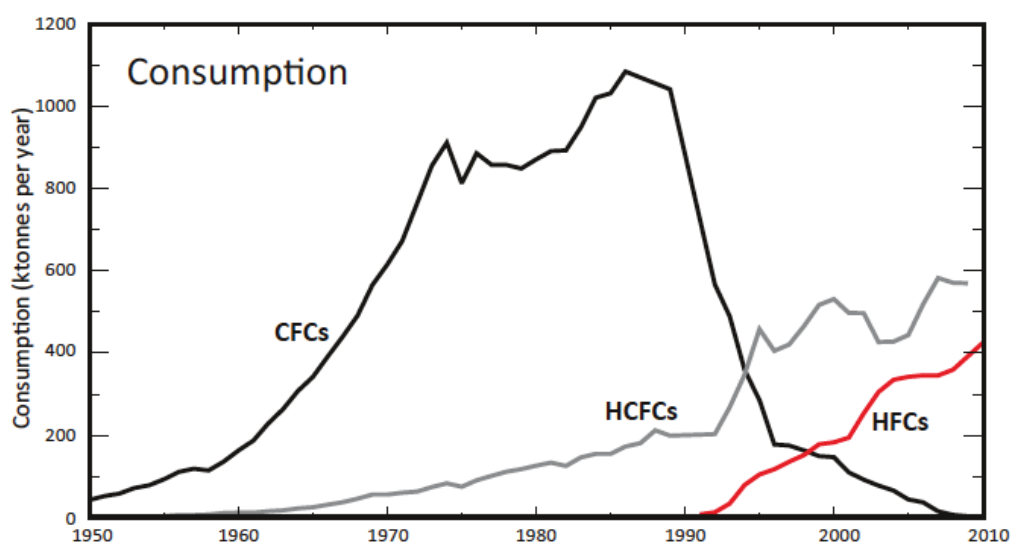
Figure 1: Increase in HFCs due to phase-out of CFCs and HCFCs
